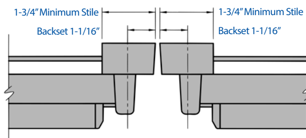
Two Concealed Vertical Rod Devices
